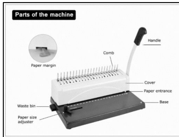
Rajah 2: Bahagian-Bahagian Binding Machine
